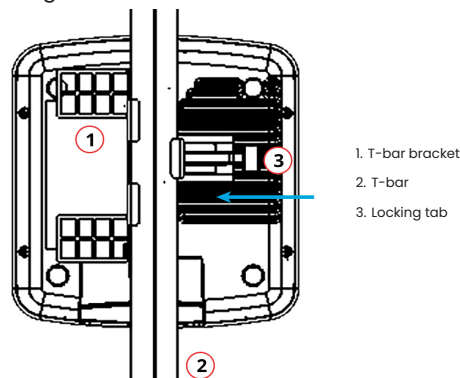
FIGURE 5 Attaching the AP and T-bar Bracket with the Locking Tab
