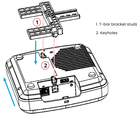
FIGURE 4 Attaching the T-bar Bracket to the AP
