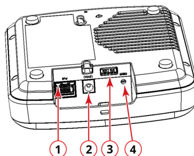
FIGURE 2 A350 AP Ports on Bottom Panel
