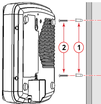
FIGURE 3 Flat Surface Mounting
